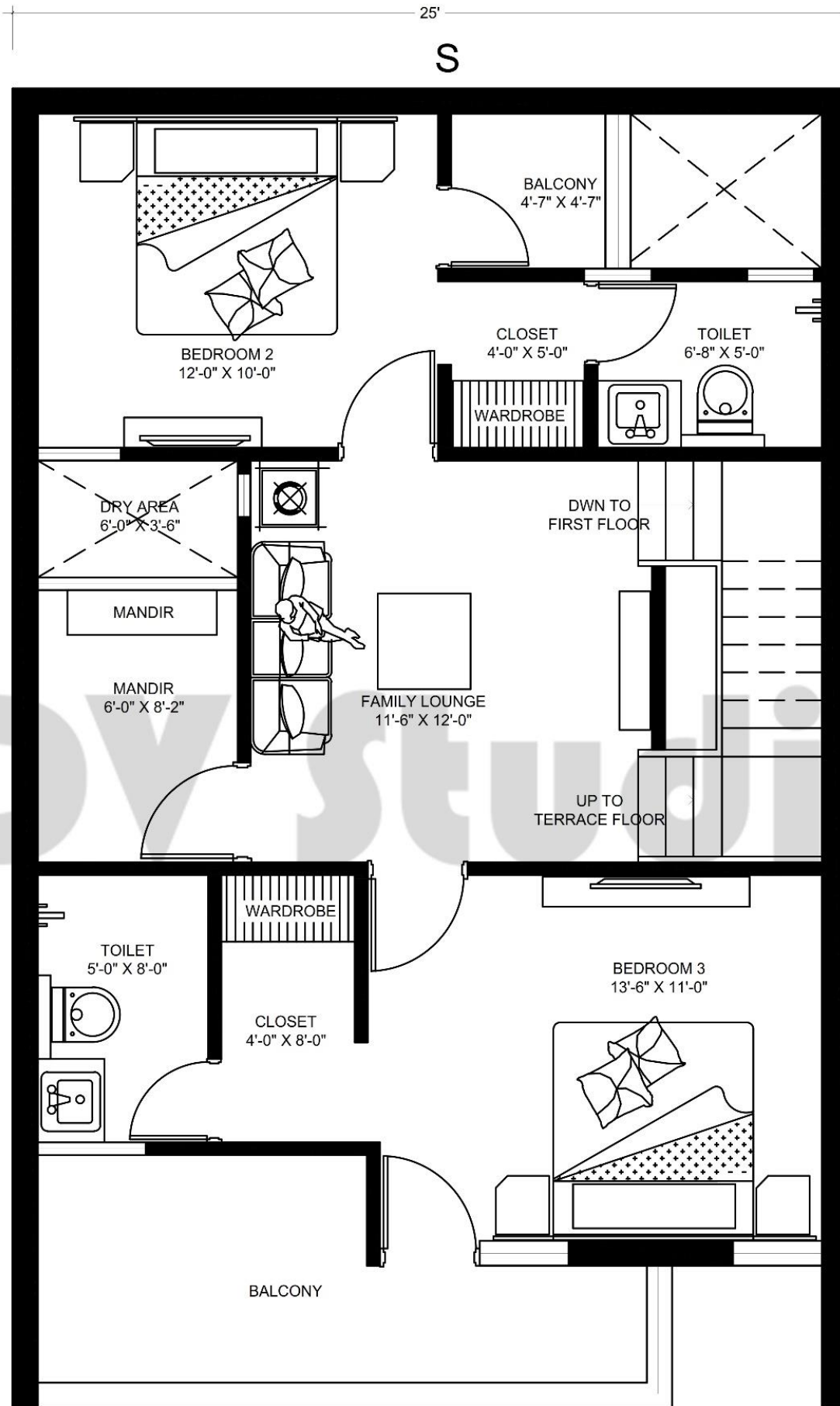
FIRST FLOOR
